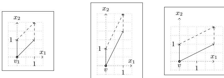
Fig. 2: Parallelepipeds for two unimodular cones and one non-unimodular cone. The last parallelepiped contains integer point (1\ 1) .
